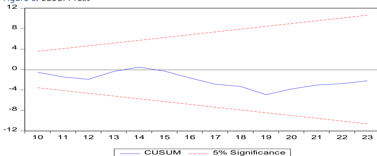
Figure 6: CUSUM Test
